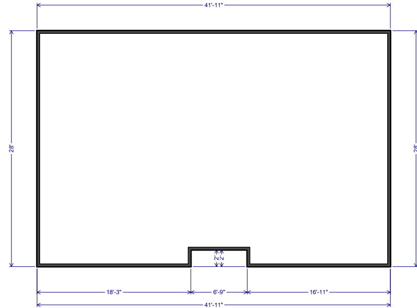
MAIN LEVEL
